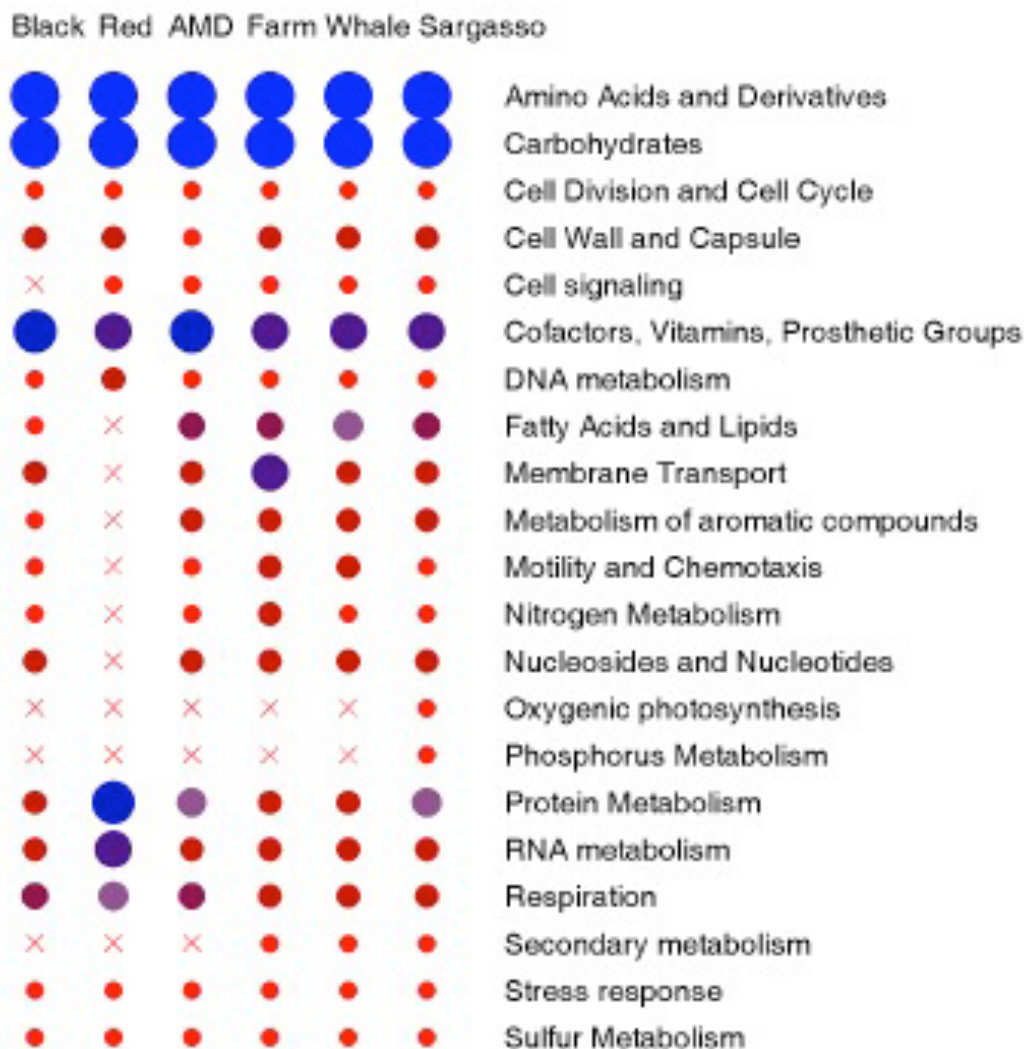
Figure 4 Subsystems present in different metagenome sequences. The subsystems present in the Sudan samples, the Iron Mountain AMD sample, the Minnesota Farm and the Sargasso Sea are shown grouped by family. The red x corresponds to very low abundance or complete absence of that family of subsystems. The size of the circle represents the proportion of sequences seen within that family of subsystems.
